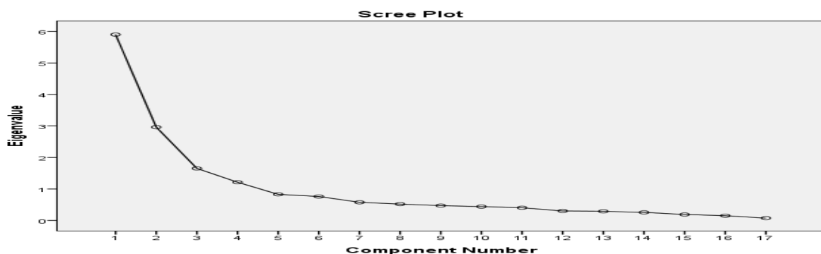
Figure 2: Scree plot of PLSE items
